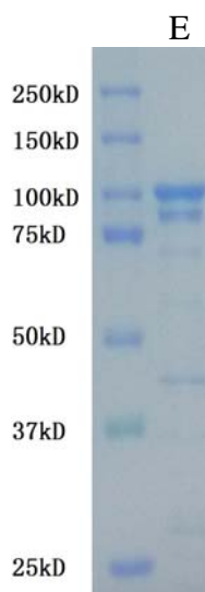
E: nsP3 (Ross River virus), partial degradation is observed.
